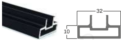
VERTICAL PROFILE (32 x 10 MM)
