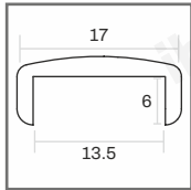
(17 x 6 MM)
