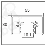
(30 x 55 MM)
