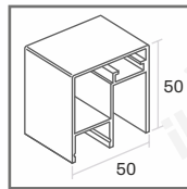
(50 x 50 MM)
