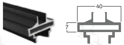
HORIZONTAL PROFILE (40 x 7 MM)
