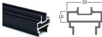
HORIZONTAL PROFILE (32 x 10 MM)
