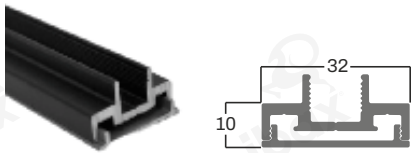
OC VERTICAL PROFILE (1+1) (32 x 10 mm)
