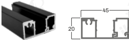
IPC 02 FOLDABLE (45 x 20 mm)
