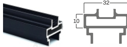
HORIZONTAL PROFILE (32 x 10 MM)
