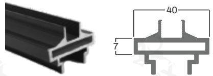
HORIZONTAL PROFILE (40 x 7 MM)
