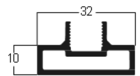
32x10 mm Series (Slim)
